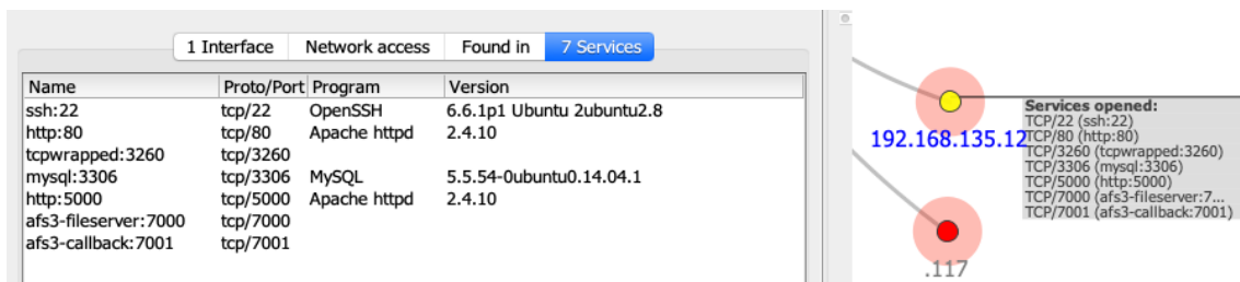
Figure 6: Showing port and service information from a Nmap report imported into a NP-View project
